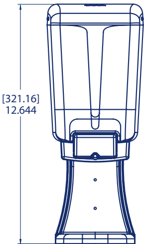
Classic soap dispenser drip tray attached to a 46 oz Classic soap dispenser
