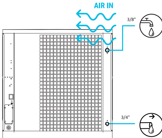
BACK VIEW
