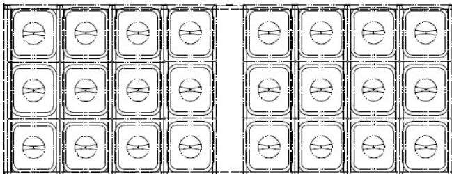
PAN LAYOUTS 24 (pcs) 1/6 pans
