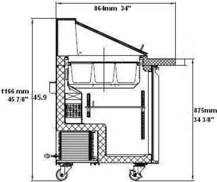
Section View
