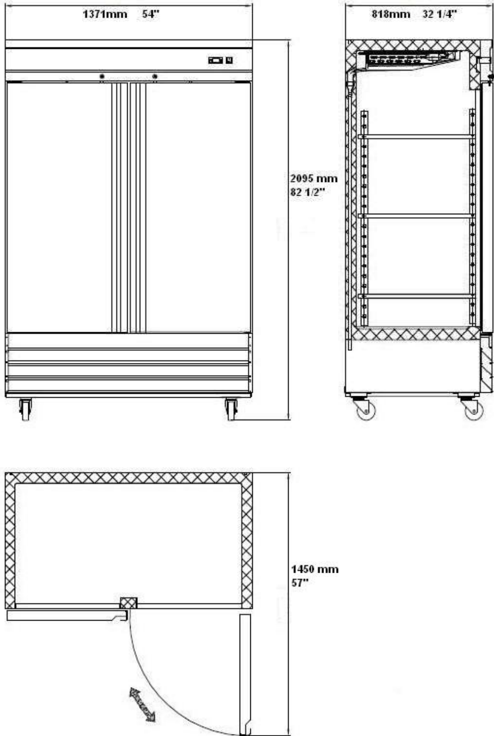
KBM2R Plan View
