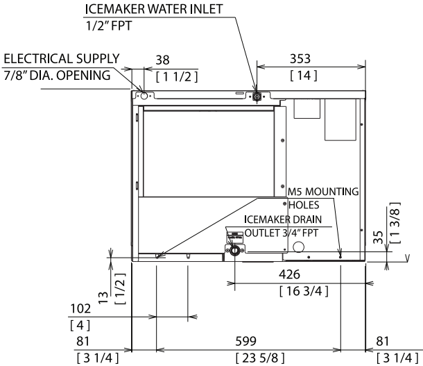
REAR VIEW
